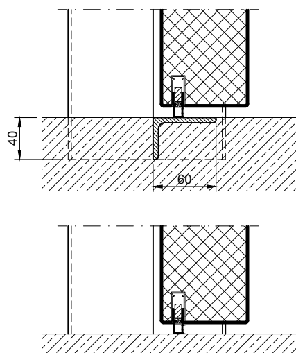
stop sill without seal
