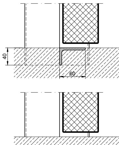
stop sill with seal
