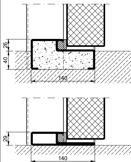
stop sill with seal
