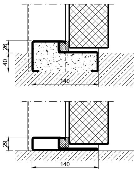
stop sill with drop seal
