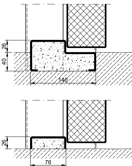
stop sill without seal
